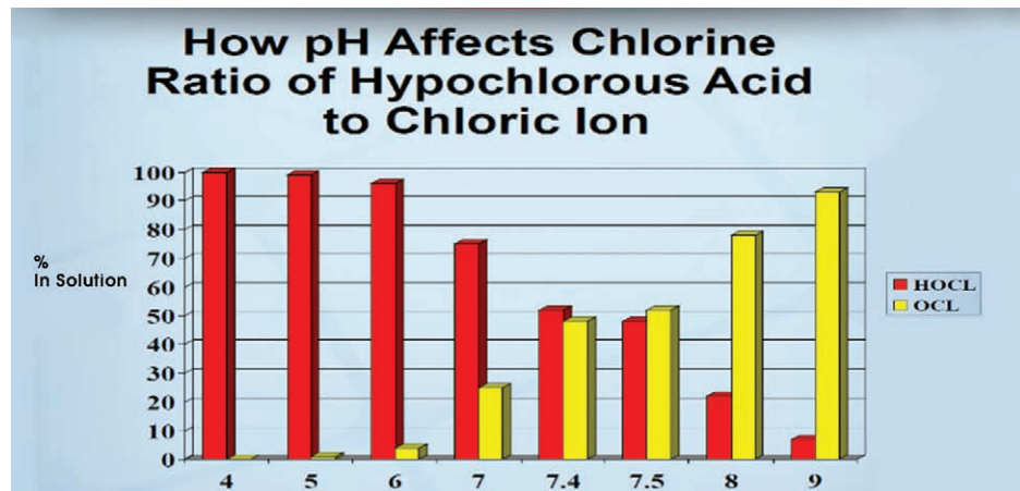
Fig. 4: pH dependent effectiveness of free chlorine
